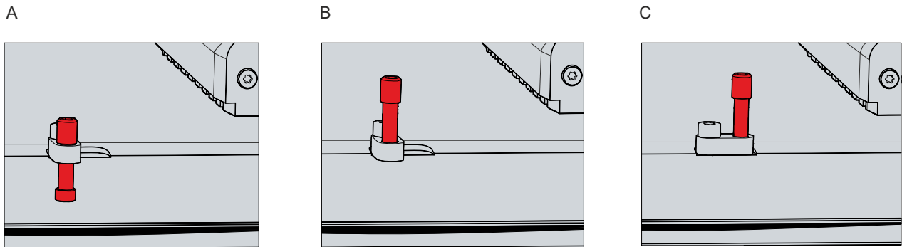
Fig. 23: CP29xx_Removal from the control cabinet
