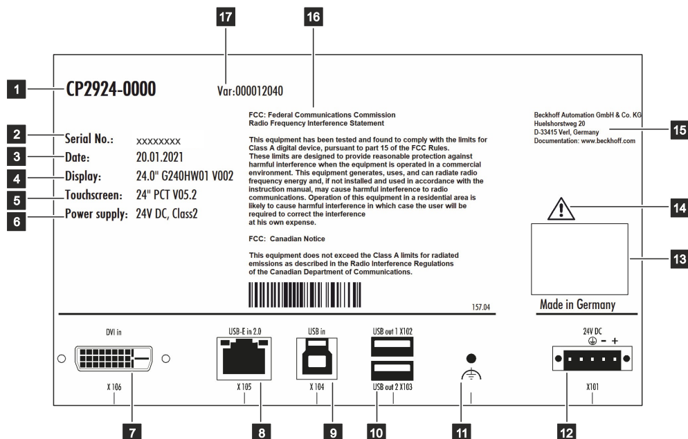
Fig. 17: CP29xx_name plate example
