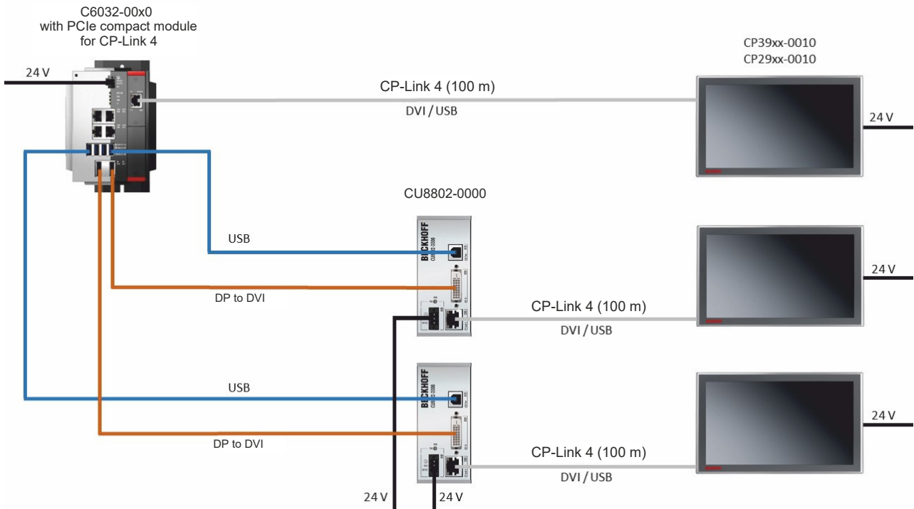
Fig. 13: CP29xx-0010_CP-Link 4, CU8802
