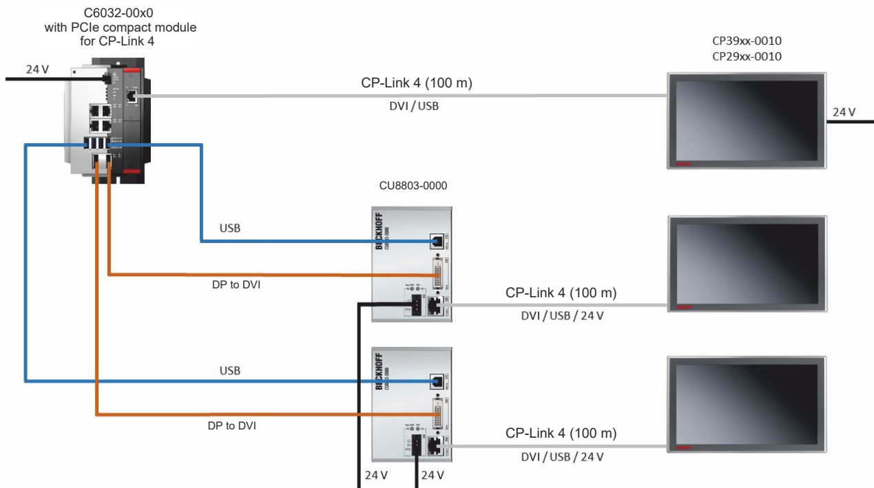
Fig. 14: CP29xx-0010_CP-Link 4, CU8803
