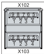
Fig. 5: CP29xx_USB interface pin numbering
