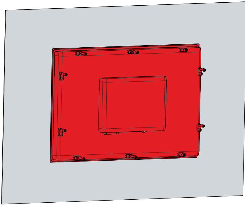
Fig. 19: CP29xx_wall positioning
