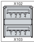
Fig. 10: CP29xx_USB interface pin numbering
