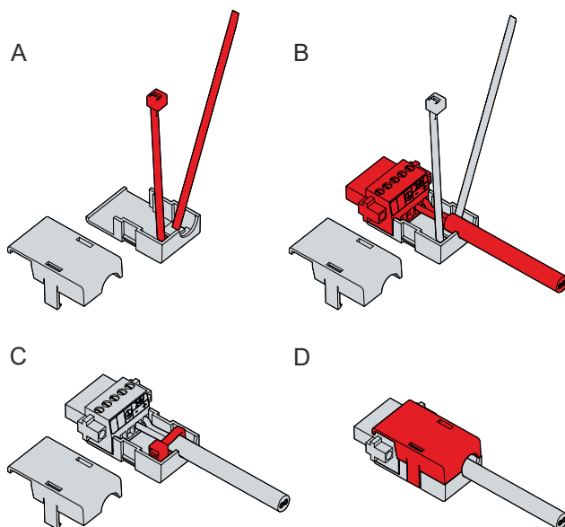
Fig. 21: CP29xx_Assembly of strain relief housing
