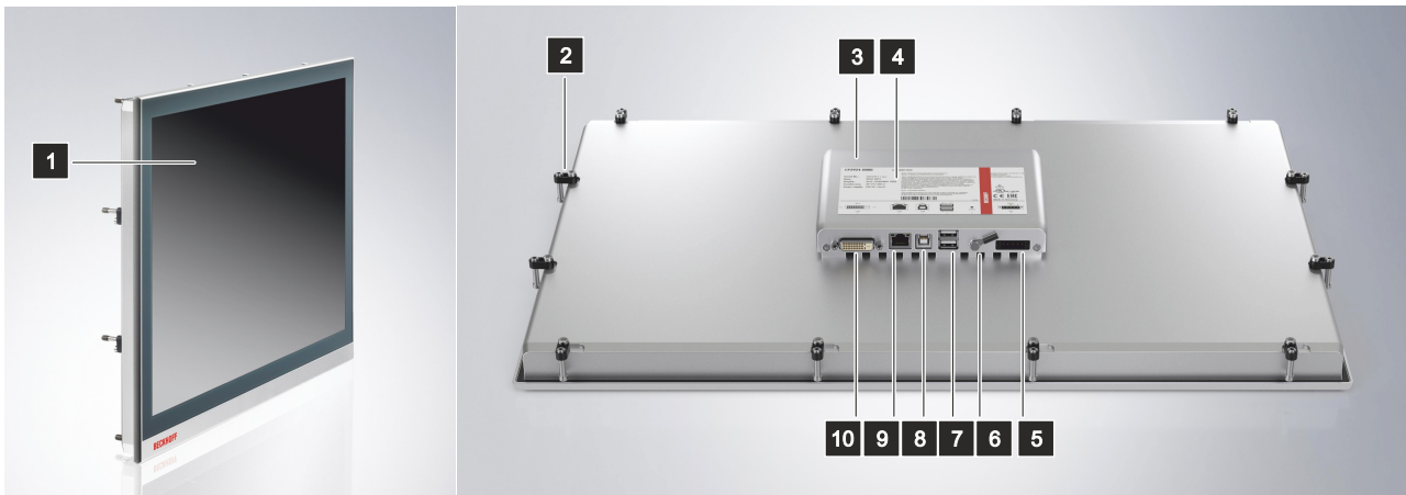
Fig. 2: CP29xx_Structure
