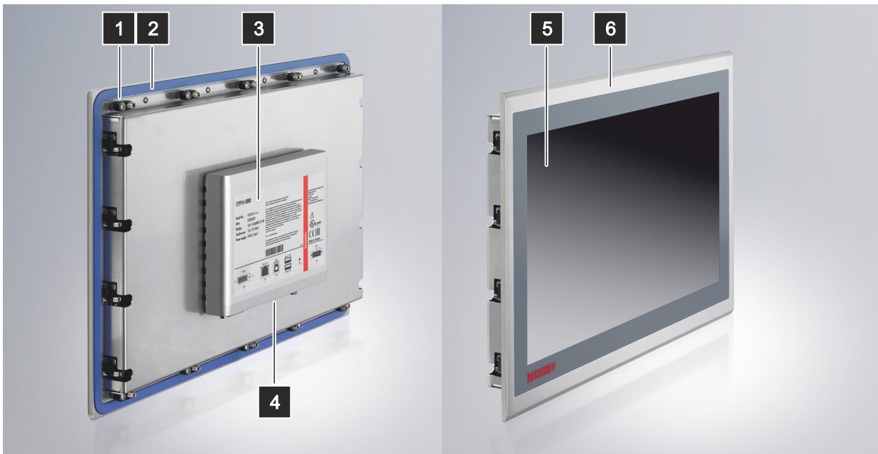
Fig. 3: CP29xx_structure stainless steel device
