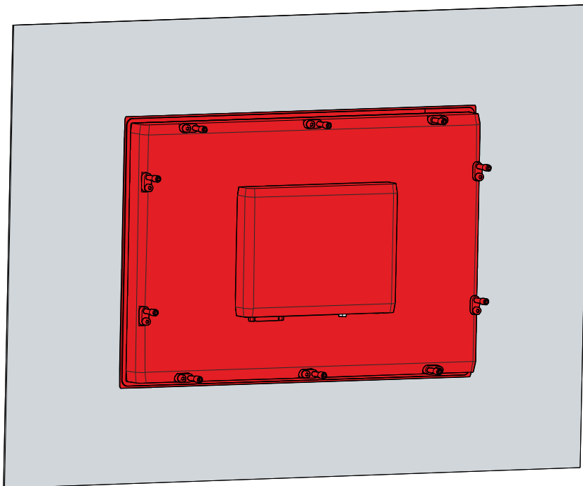
Fig. 24: CP29xx_removal installation cutout
